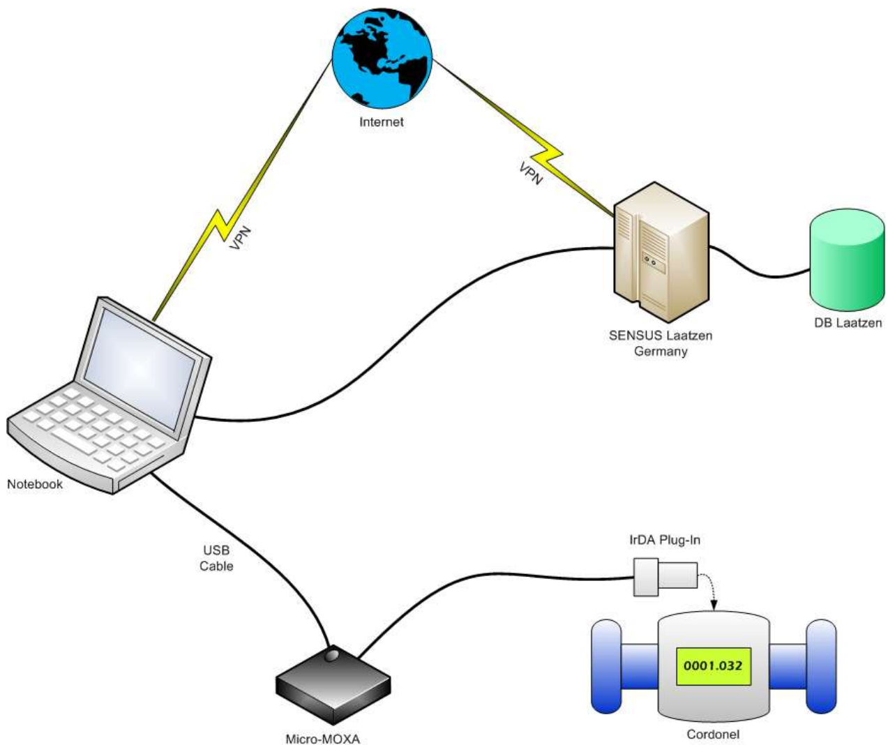
Figure 4.1 System Connections
