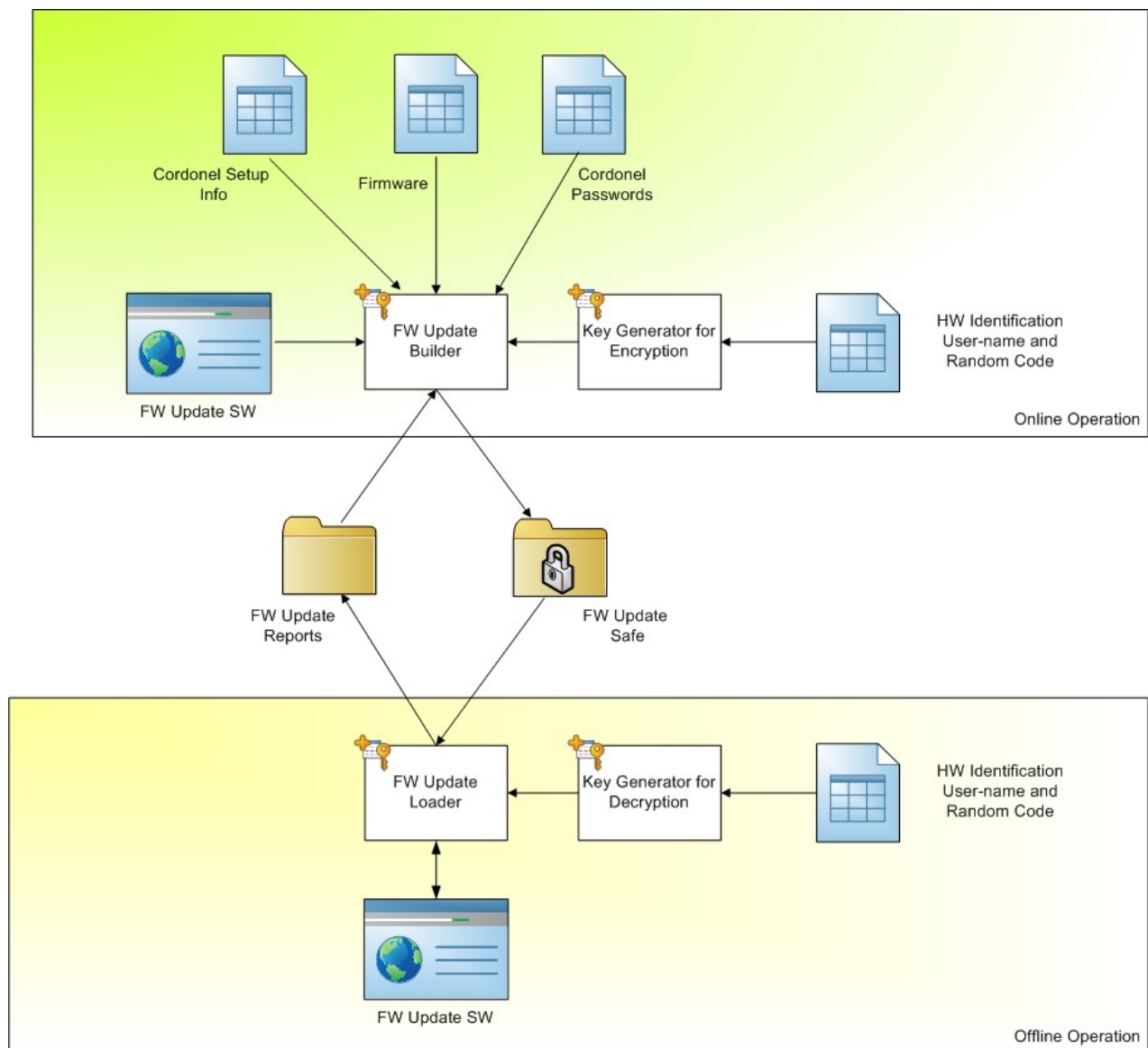
Figure 4.2 System Overview
